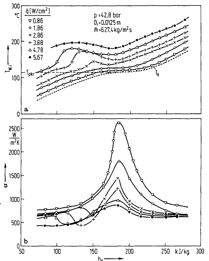
Fig. 4a and b. Heat transfer impairment under different heat flux densities. a wall temperature, b heat transfer coefficient
