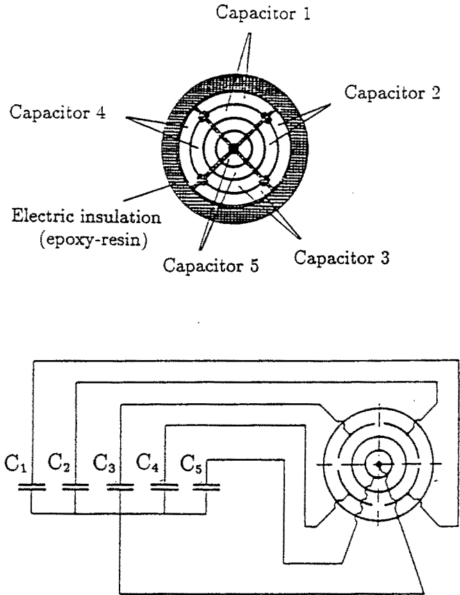
Figure 2. Impedance void meter
