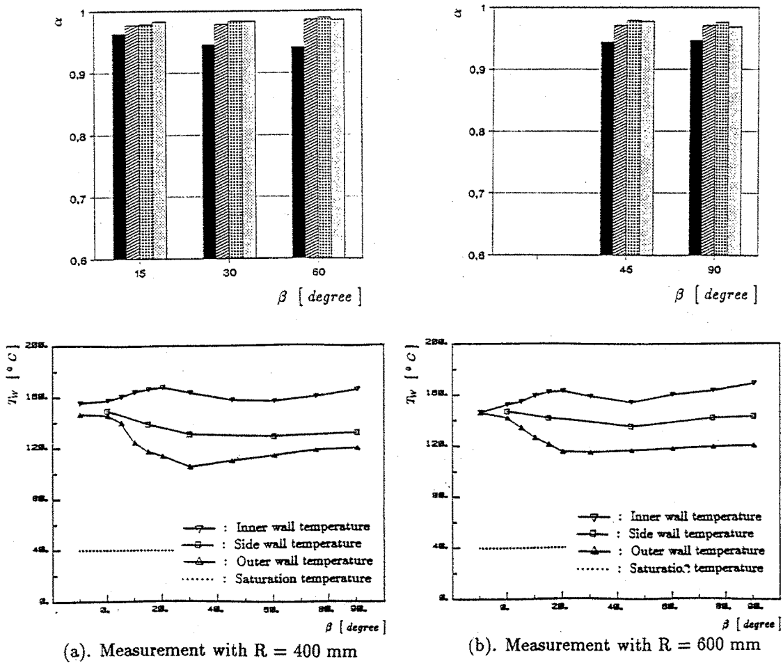
Figure 8. Void fraction and temperature distributions in bends at: P = 9.5 bar, G = 400 kg/m 2 s, q''_w = 30 kw/m 2
