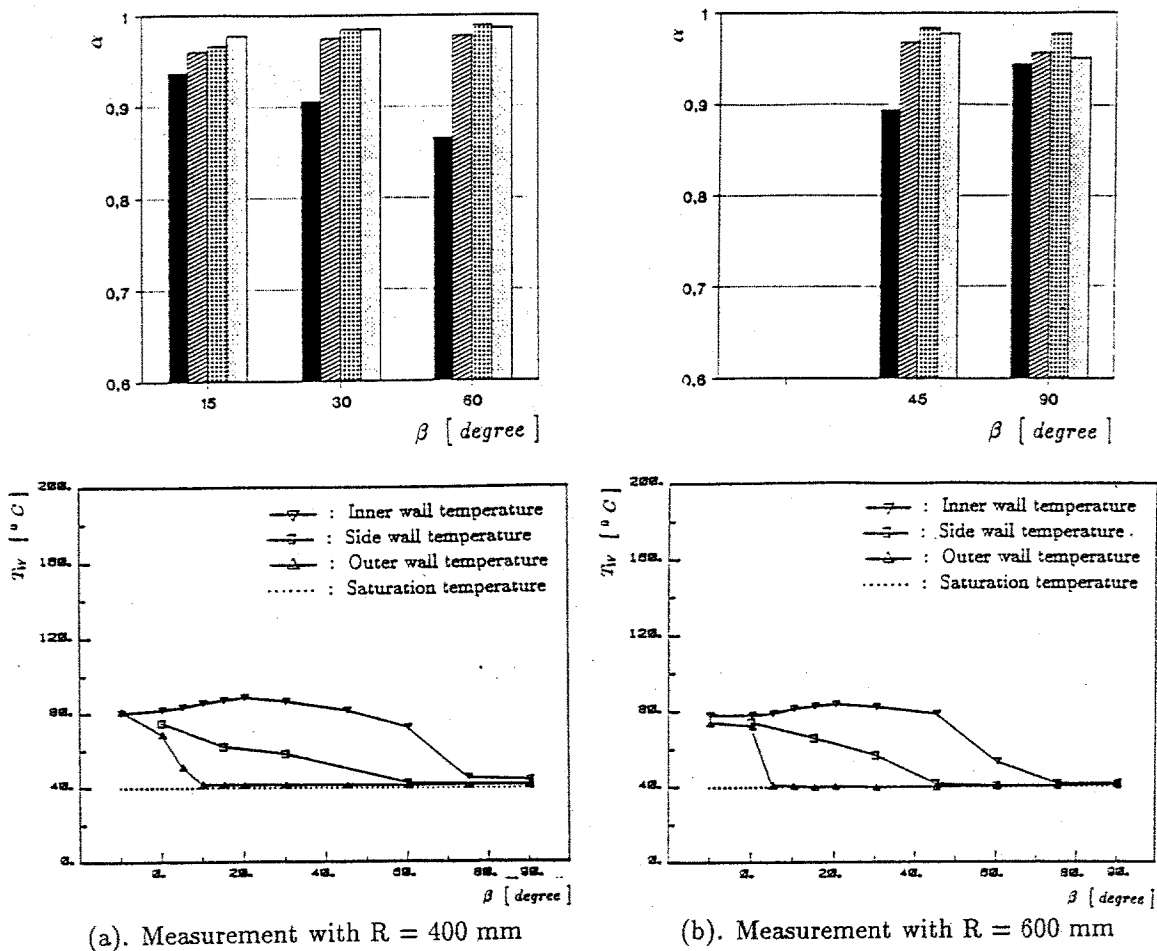
Figure 9. Void fraction and temperature distributions in bends at: P = 9.5 bar, G = 1200 kg/m 2 s, q''_w = 30 kW/m 2
