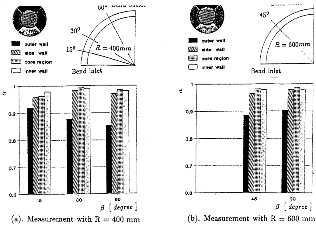
Figure 7. Void fraction distributions in bends at: P = 9.5 bar, G = 680 kg/m 2 s, q''_w = 50 kw/m 2
