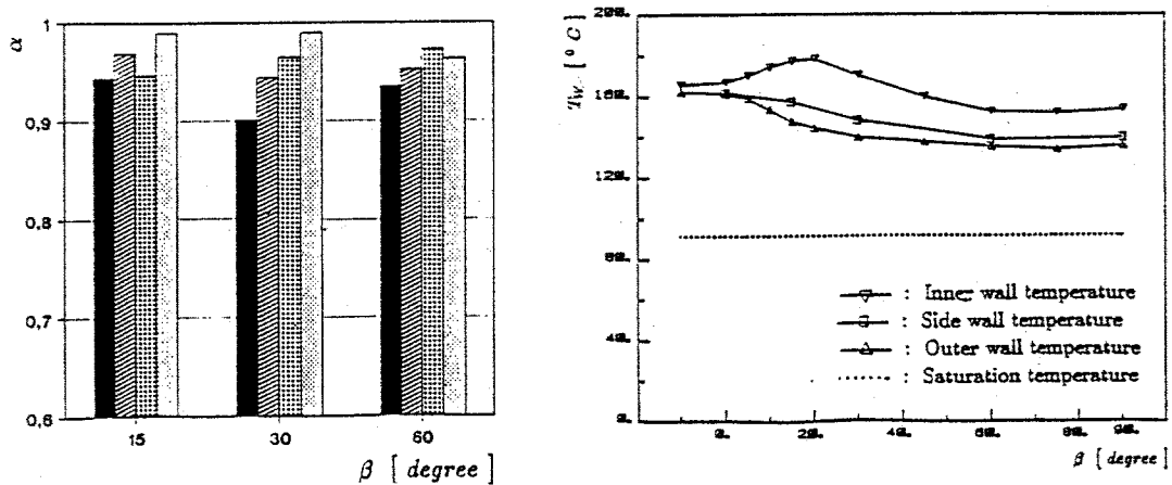
Figure 10. Void fraction and temperature distributions in bend with R = 400 mm at: P = 28.5 bar, G = 400 kg/m 2 s, q''_w = 30 kW/m 2
