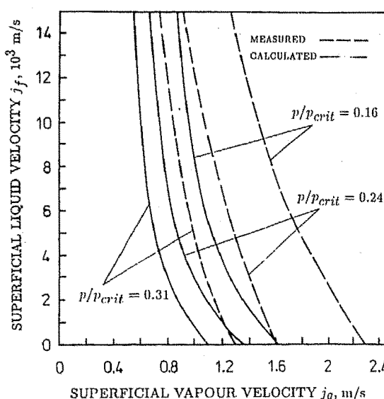
Fig. 13. Measured and empirically calculated flooding curves (conditions of present R 12 tests. Curves calculated using Eq. (19)).
