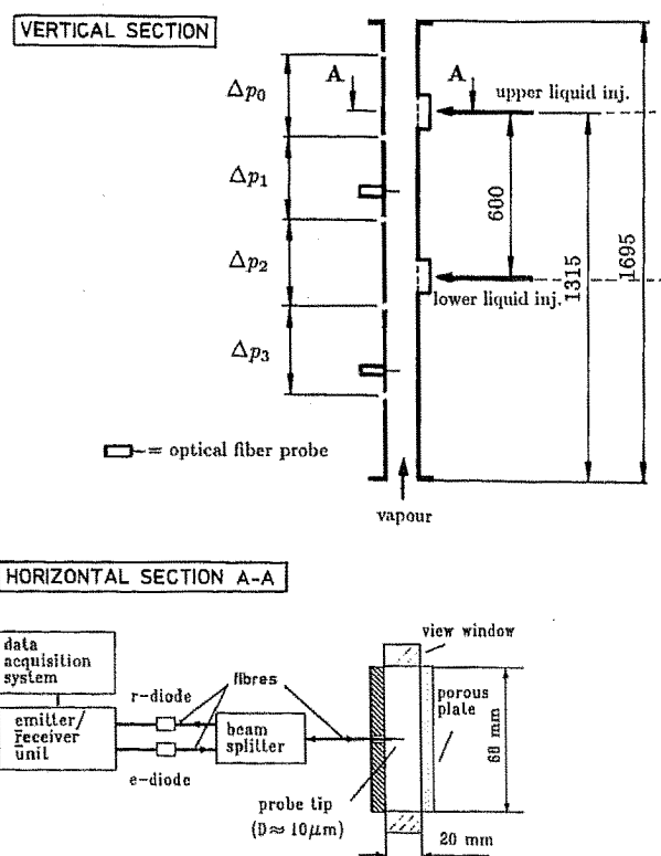
Fig. 3. Test section and optical fibre probe set-up.
