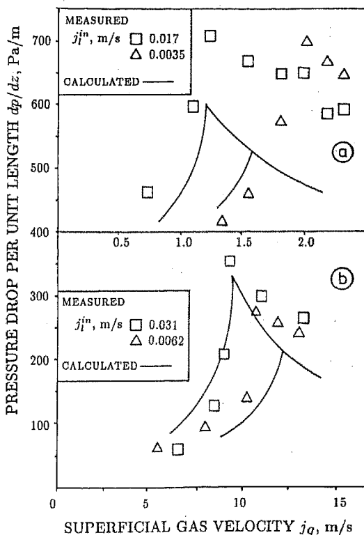
Fig. 15. Measured and analytically calculated pressure drop in counter-current flow region (a: conditions of present R 12 tests at p = 0.67 MPa, b: conditions of air/water tests of Zabarar [13]; f_i according to Eq. (18)).
