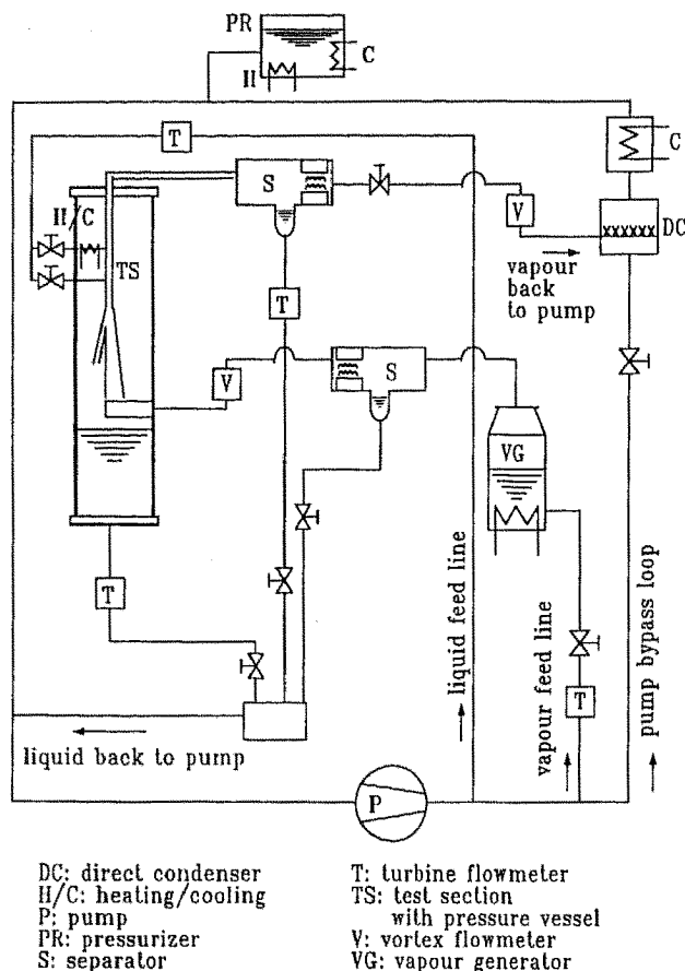
Fig. 2. Schematic diagram of test loop.
