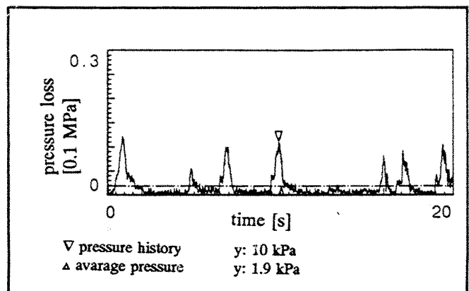
Fig.12 Plot of pressure loss across the test section with oil and air at medium level gas volume rate (Point 5) and 30 degrees valve opening
