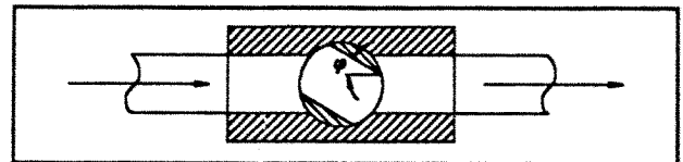
Fig.3 Cut through the ball valve with a closing angle \phi of 30 degree
