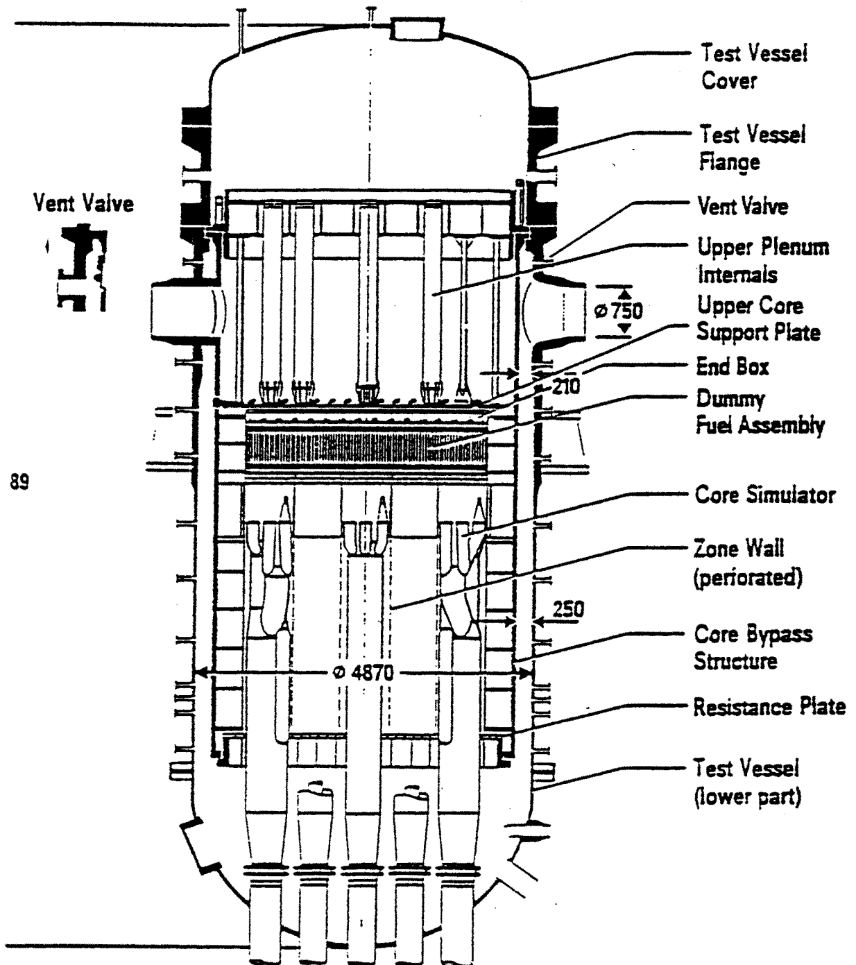
TF-Test Vessel and its Internals
