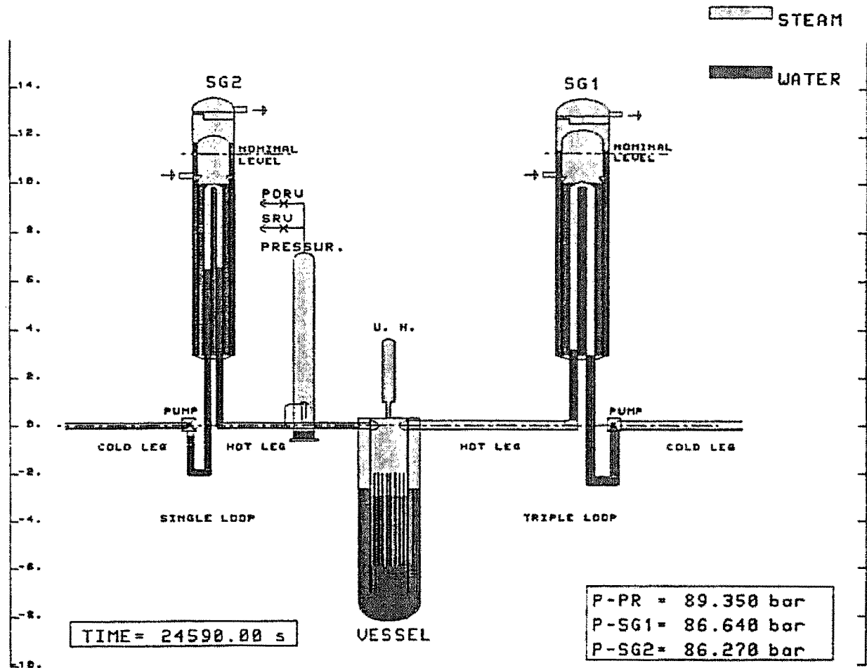
Figure 11. Fluid distribution at 56% coolant inventory.
