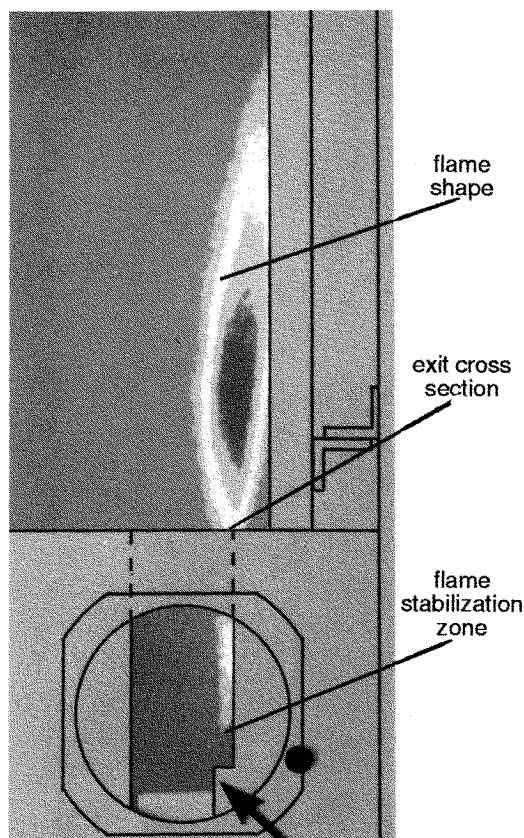
FIG. 7. Image of the reaction front distribution of a high-speed hydrogen/air flame recorded by means of OH self-fluorescence ( M_\infty = 0.93 , single hole injector, \alpha = 45^\circ , (\rho w)_{H_2} = 159.2 \text{ kg m}^{-2} \text{ s}^{-1} ).
