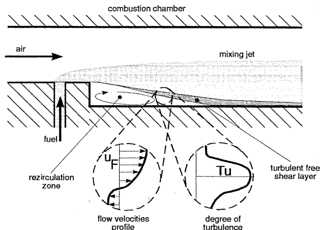
FIG. 10. Sketch of the flow field in the vicinity of the injection zone and rearward facing step.
