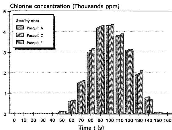
Figure 5 Time plots of the chlorine concentration at the location marked as X (see Figure 4) for three different atmospheric stability classes (A: unstable; C: indifferent; F: stable stratification); wind coming from the south
