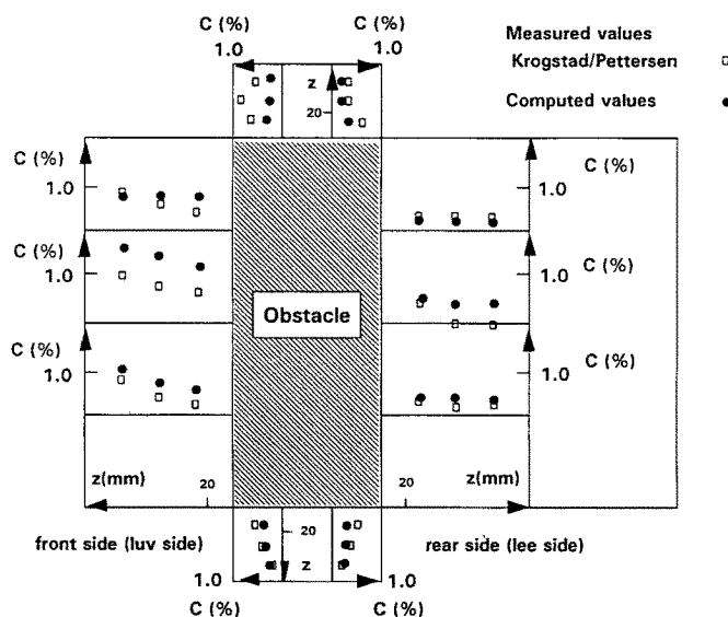
Figure 1 Comparison between computed (●) and measured (□) values for the Freon R12 concentration on an obstacle's side walls (continuous R12 release; experimental data from Reference 14, computations using the present method)
