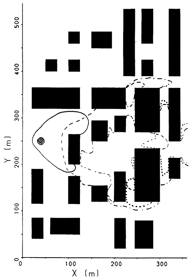
Figure 3 Temporal development of the 40 ppm chlorine iso-concentration line on a z-plane at height 2.5 m above ground; wind coming from the west: (—) 10 s; (---) 70 s; (- - -) 130 s; (· · ·) 180 s after release
