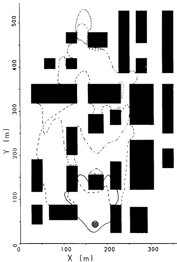
Figure 2 Temporal development of the 40 ppm chlorine iso-concentration line on a z-plane at height 2.5 m above ground; wind coming from the south: (—) 10 s; (---) 70 s; (- - -) 130 s; (· · ·) 180 s after release
