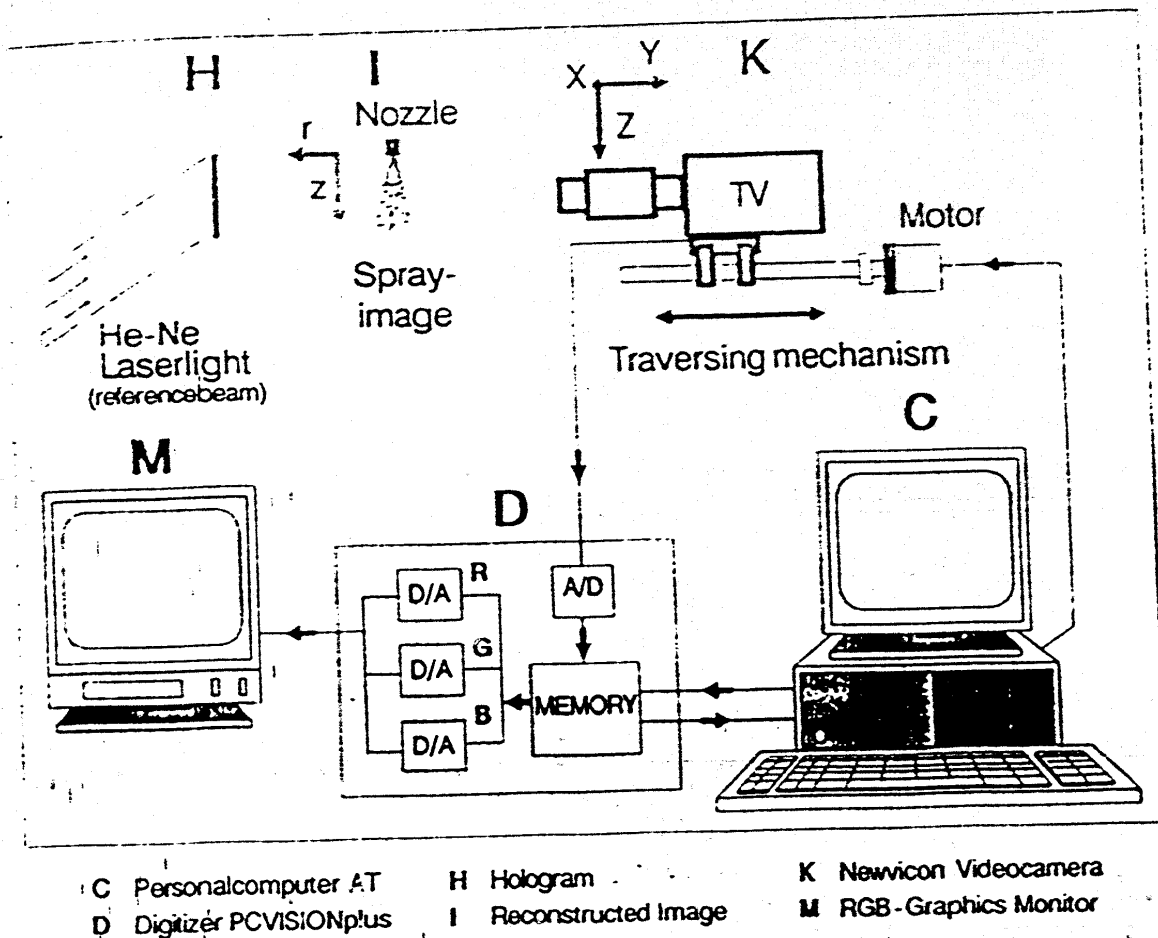
Fig. 9: Digital image processing system for the evaluation of pulsed laser holograms
