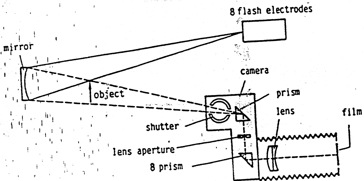
Fig. 3: Cranz-Schardin-camera for ultra short-time cinematography
