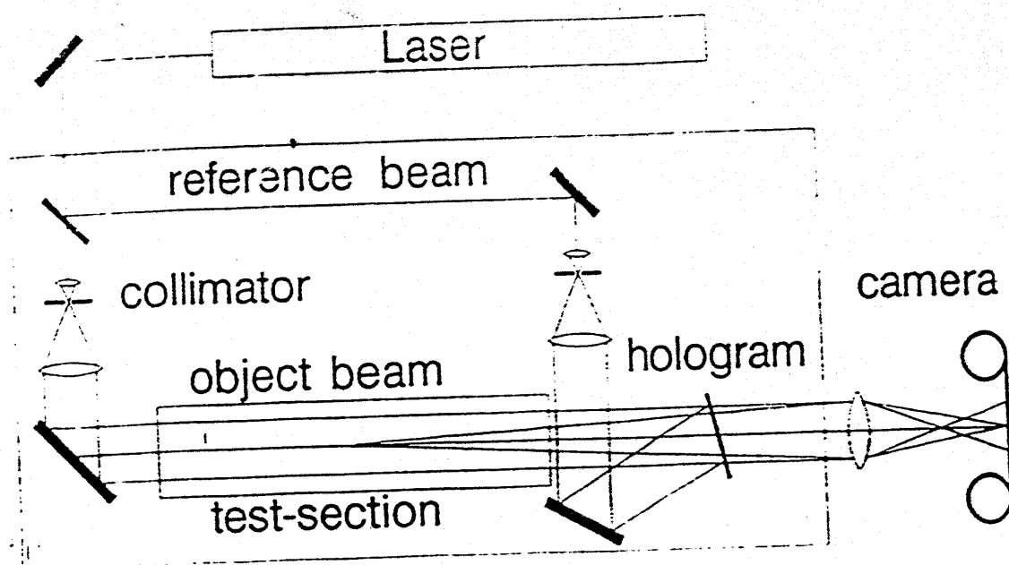
Fig. 14: Optical set-up for holographic interferometry
