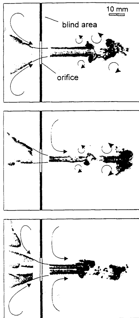
Fig. 11: Igniting phenomena resulting from a jet of burnt hydrogen and radicals in hydrogen-air-mixture
