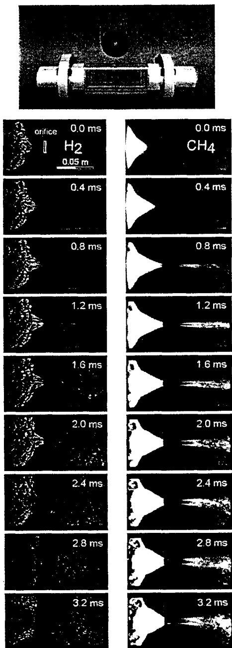
Fig. 10: Flame formation in front and after an orifice with H_2 and CH_4 as combustible.
