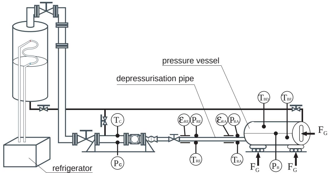
Abbildung 1: Test facility
