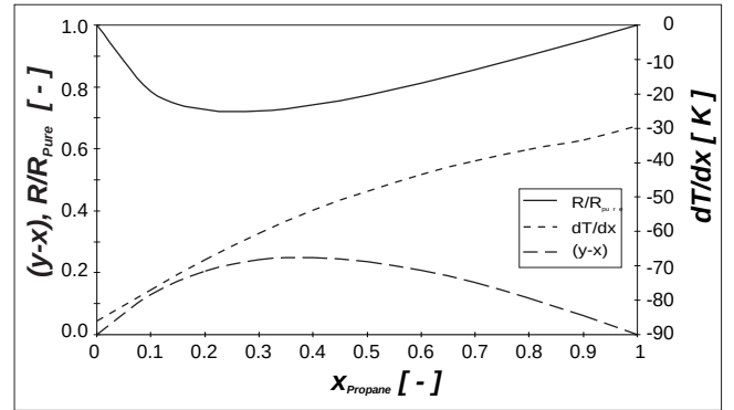
Abbildung 5: Reduced bubble growth of a Propane/Butane binary mixture in comparison to a pure fluid
