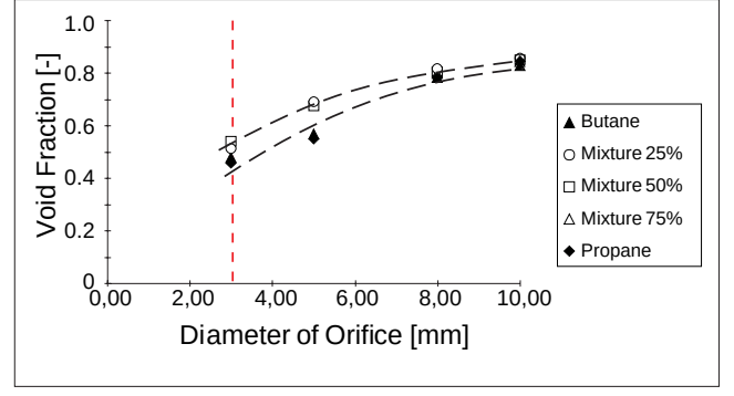
Abbildung 10: Measured Void Fraction at the Pipe Exit in Dependence of Composition and Diameter of Orifice
