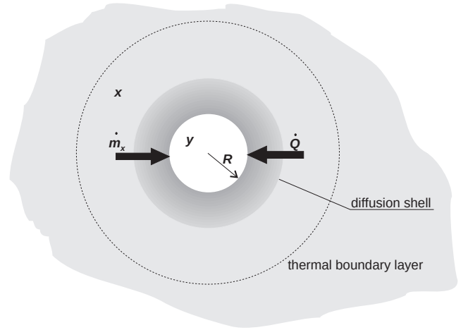
Abbildung 4: Thermal boundary layer and diffusion shell around a growing bubble
