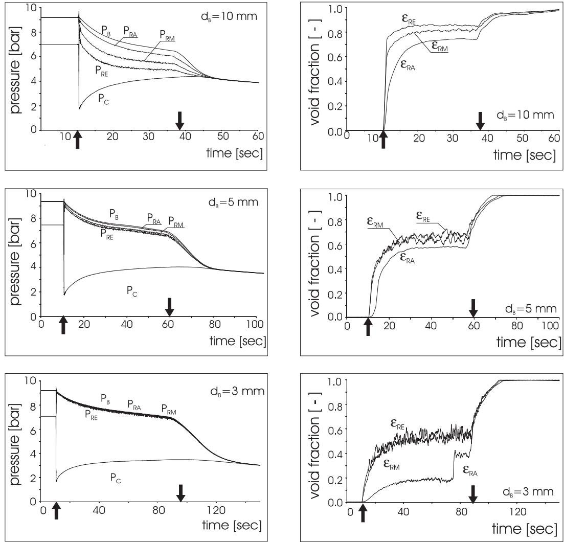
Abbildung 7: Influence of Diameter of Orifice, Propane/Butane Binary Mixture (50mol%), L/d = 240
