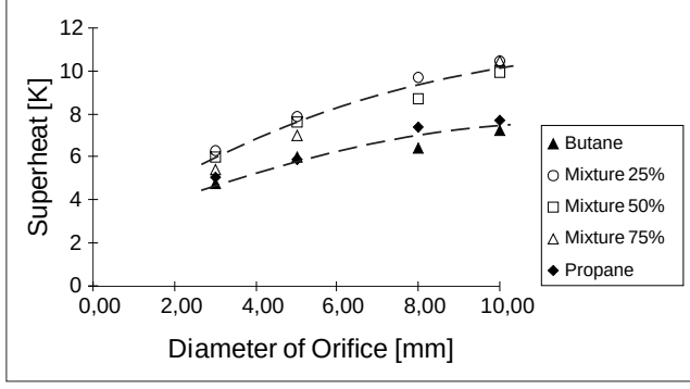
Abbildung 8: Thermal Non-Equilibrium in Vessel in Dependence of Composition and Diameter of Orifice
