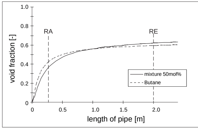
Abbildung 11: Comparison of the void fraction development for a pure fluid and a binary mixture
