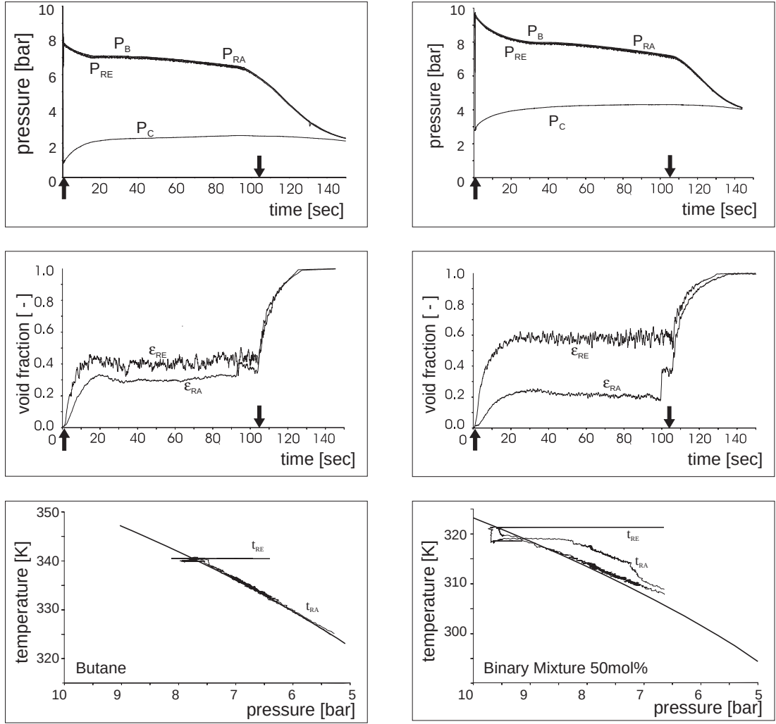
Abbildung 6: Comparison of Fluids: Butane and a Propane/Butane binary mixture (50mol%), L/D = 170 , d_B = 3\text{ mm}
