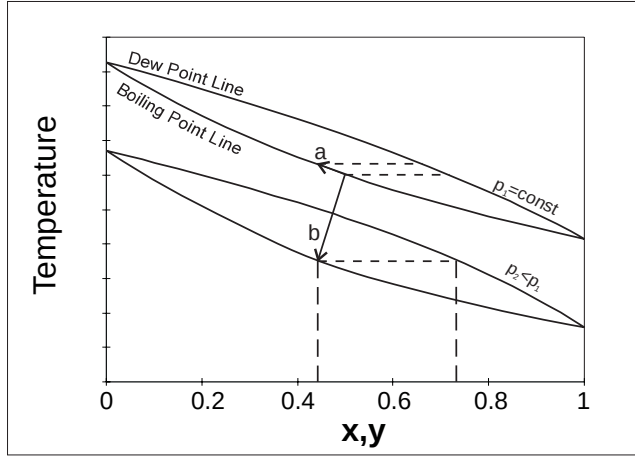
Abbildung 3: Phase equilibrium diagram: Decrease of the local concentration of the more volatile component
